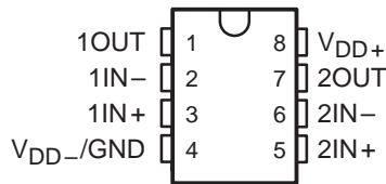
TLC2262M, TLC2262AM . . . JG PACKAGE (TOP VIEW)
